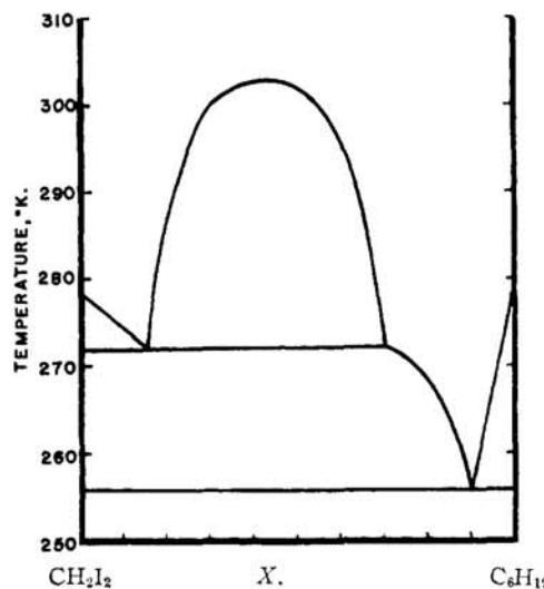
Fig. 3A.—Calculated phase diagram for the binary system methylene iodide-cyclohexane (using thermodynamic parameters of Table I).
