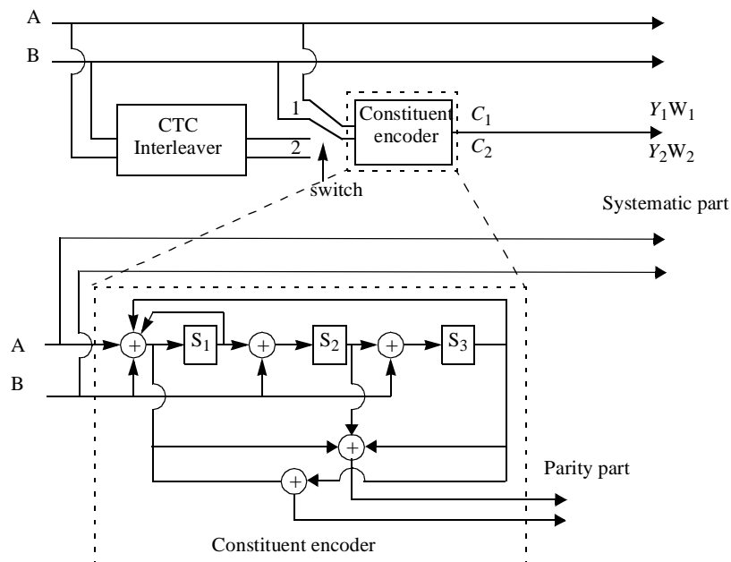
Figure 257—CTC encoder
