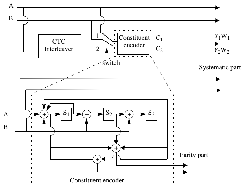
Figure 257—CTC encoder
