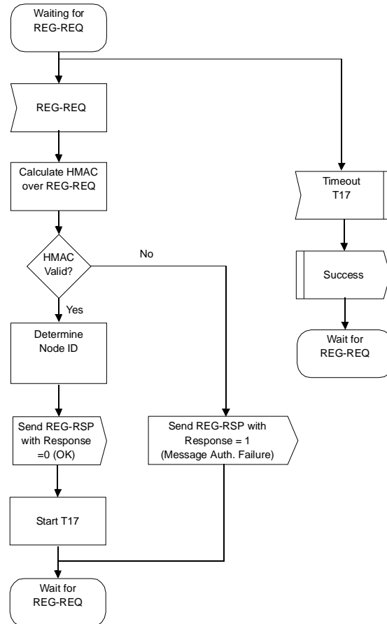
Figure 78—Registration—Registration node
