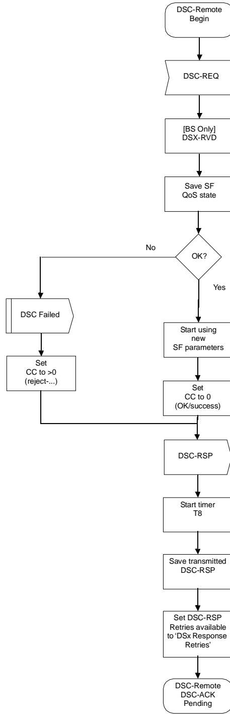
Figure 120—DSC—Remotely Initiated Transaction Begin state flow diagram
