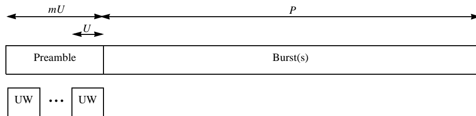
Figure 185—Base frame
