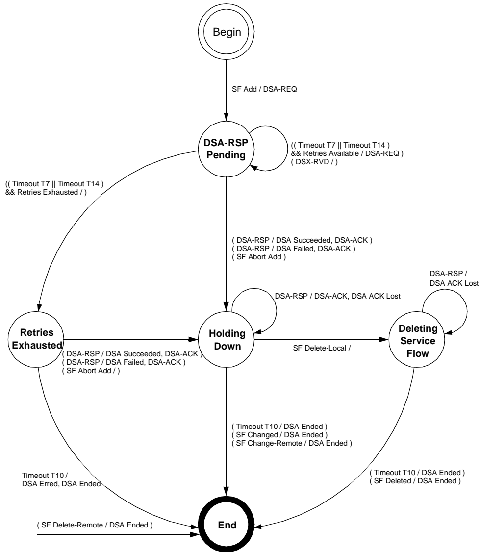
Figure 100—DSA—Locally Initiated Transaction state transition diagram
