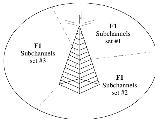
Figure B.6—Reuse of 1 configuration, 3 sectors per cell
