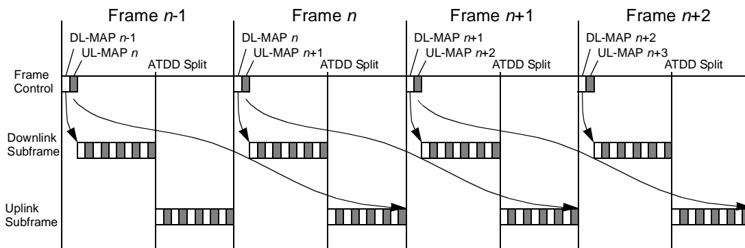
Figure 46—Maximum time relevance of DL-MAP and UL-MAP(TDD)
