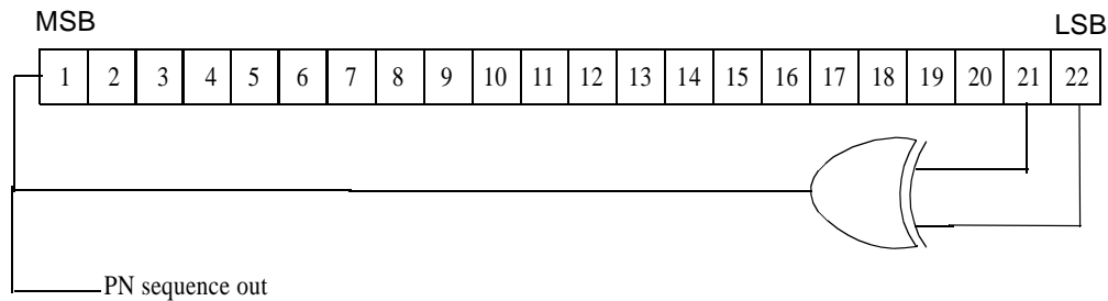
Figure 177—Spreading PN sequence generator
