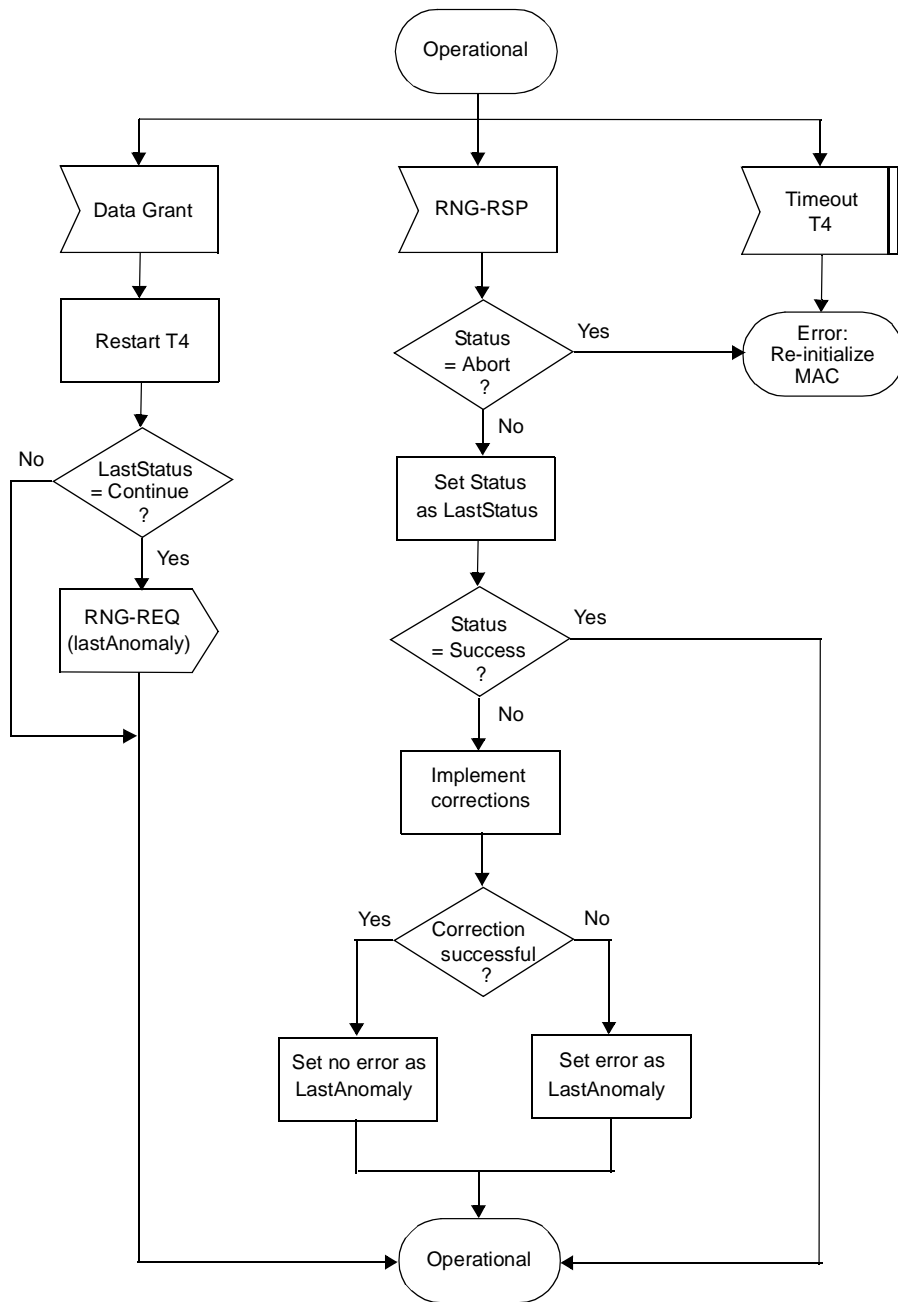
Figure 84—Periodic Ranging—SS
