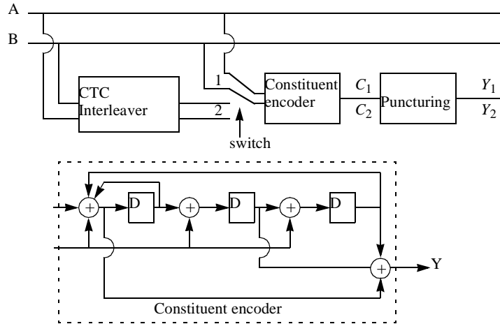
Figure 202—CTC encoder
