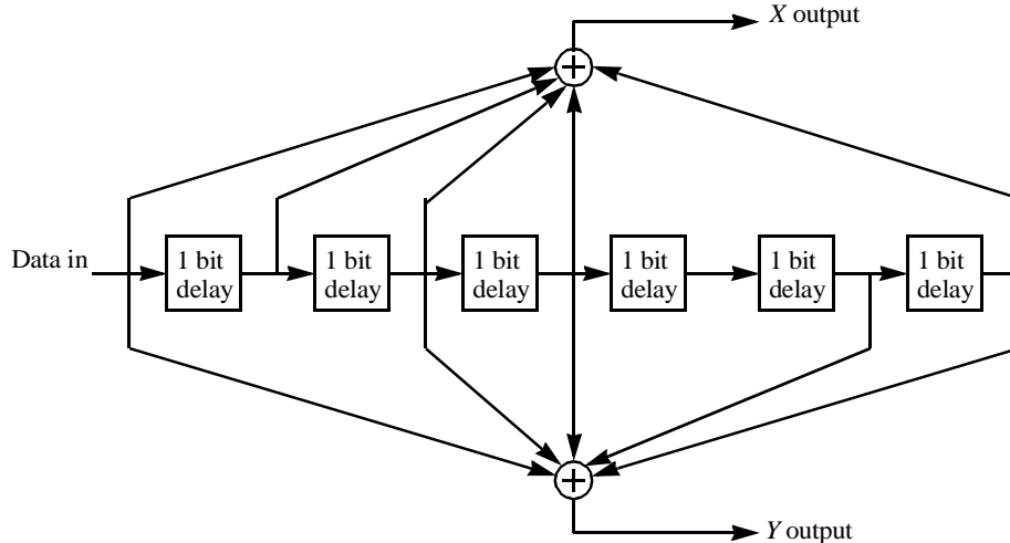
Figure 200—Convolutional encoder of rate 1/2
