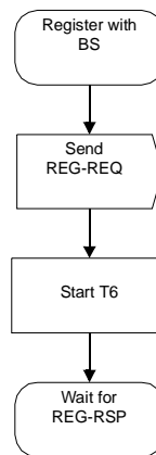
Figure 68—Registration—SS
