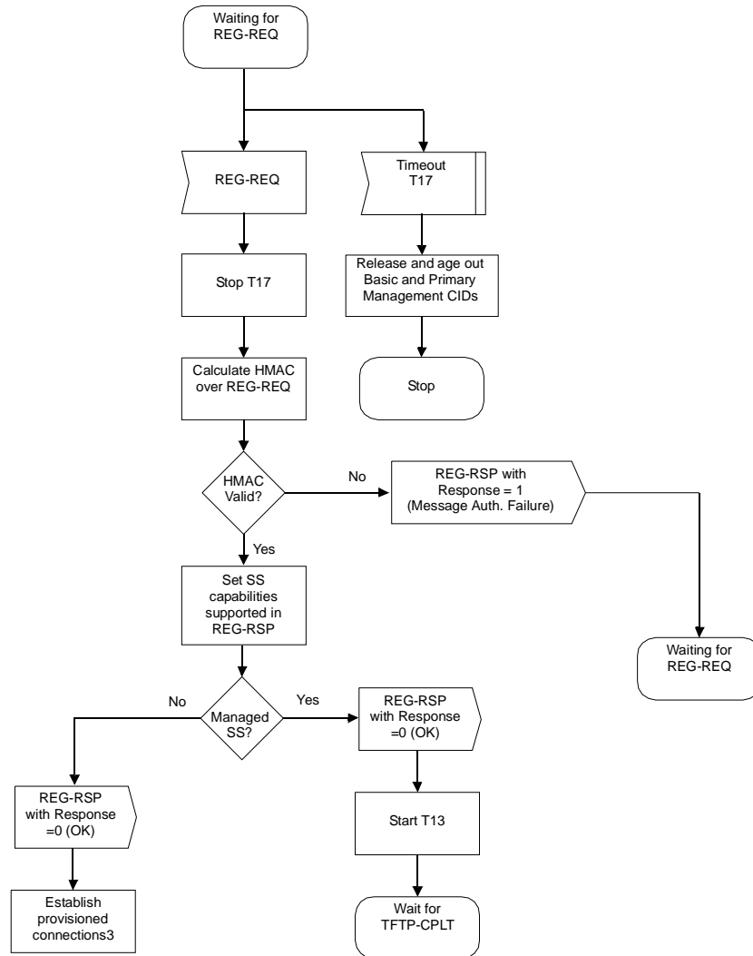
Figure 70—Registration—BS
