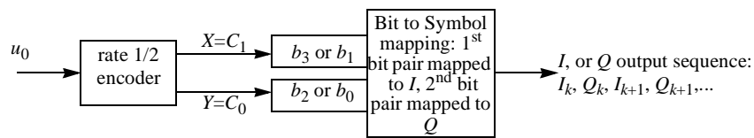
Figure 162—Pragmatic TCM encoder for rate 1/2 16-QAM
