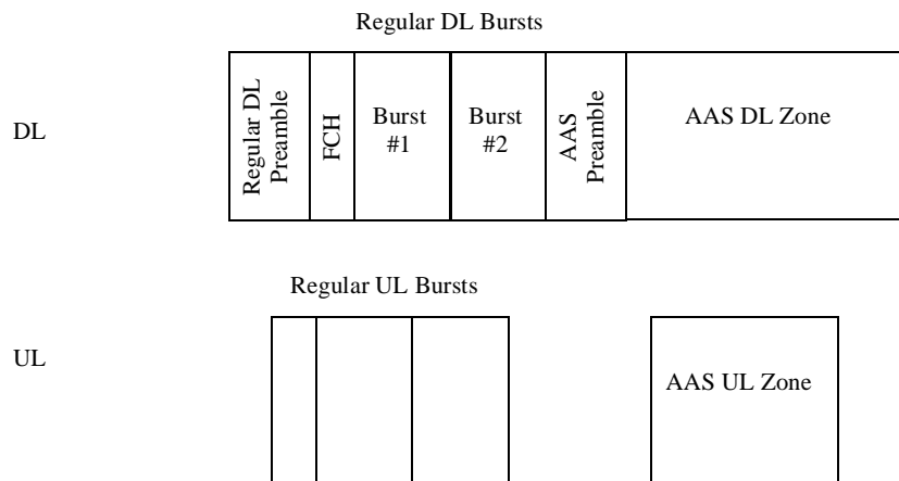
Figure 52—AAS Zone, FDD
