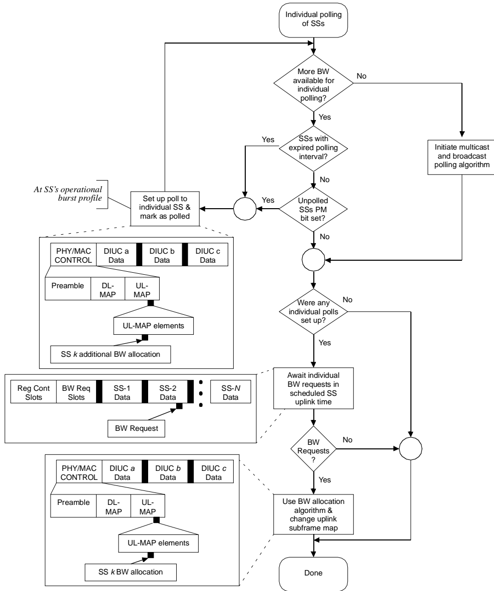
Figure 38—Unicast polling
