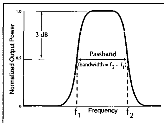
bandpass filter
