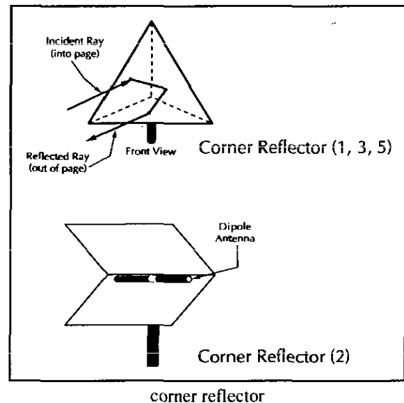
corner reflector
