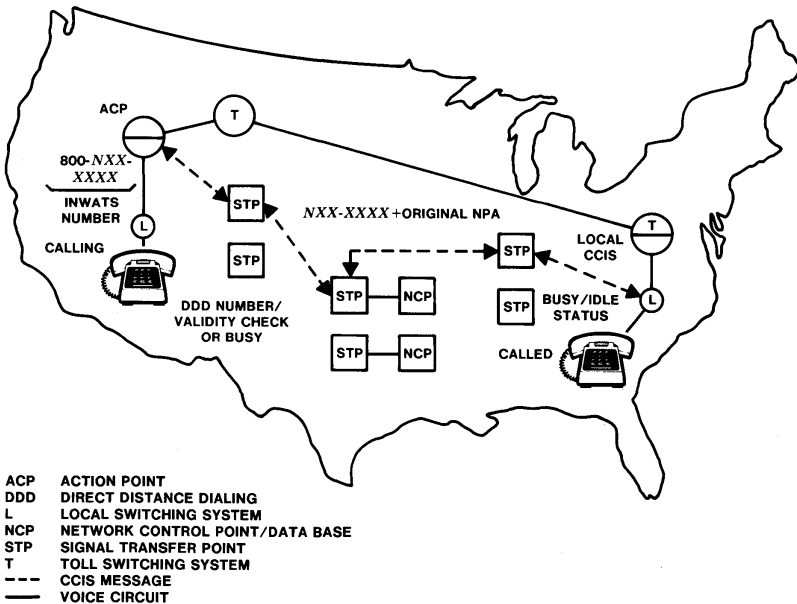
Figure 11-30. Stored-program control network—Expanded 800 Service.
