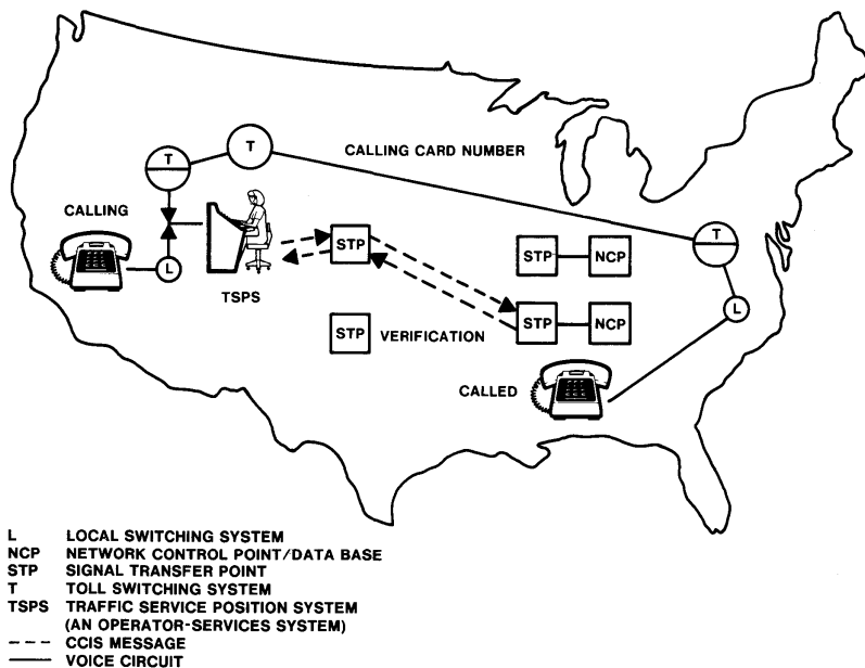
Figure 11-29. Stored-program control network—Automated Calling Card Service.
