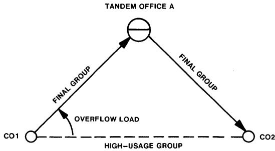
Figure 5-8. Alternate-route triangle.
