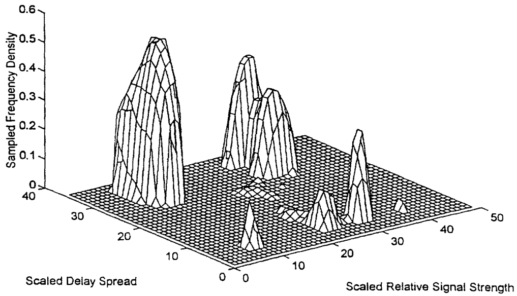
Figure [redacted]: Results of Combining Input Cropping (50% clip) with Median Filtering (4x4)
