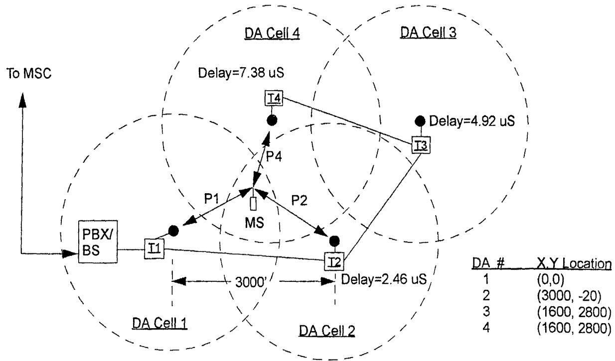
FIG. 13: DA Cell Geometry Illustration
