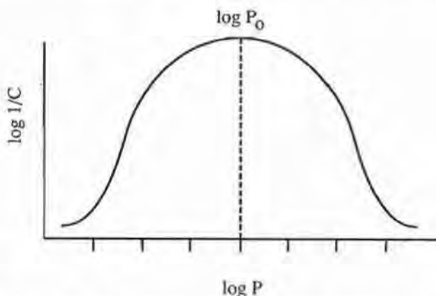
Figure 2.4. Effect of \log P on biological response. P is the partition coefficient, and C is the concentration of the compound required to produce a standard biological effect.
