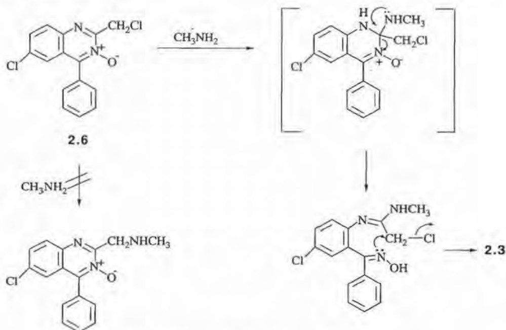
Scheme 2.1. Mechanism for formation of Librium.
