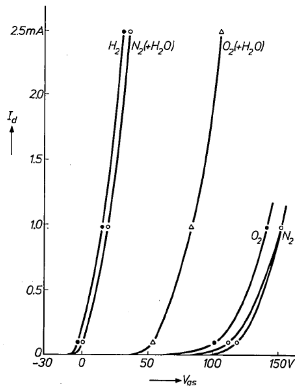
Fig. 4. The I_d - V_{gs} characteristics of a number of geometrically
