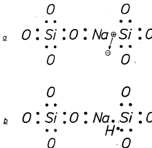
Fig. 6. a ) The location of a sodium atom in SiO 2 . The sodium atom breaks the bond between a silicon and an oxygen atom, and as a result one of the valence electrons of the silicon loses its bond; this electron is easily released and leaves behind a positive charge. b ) A hydrogen atom can introduce an SiH group in SiO 2 . In this group the hydrogen atom forms a homopolar bond with the silicon and there is no longer an unpaired electron.
