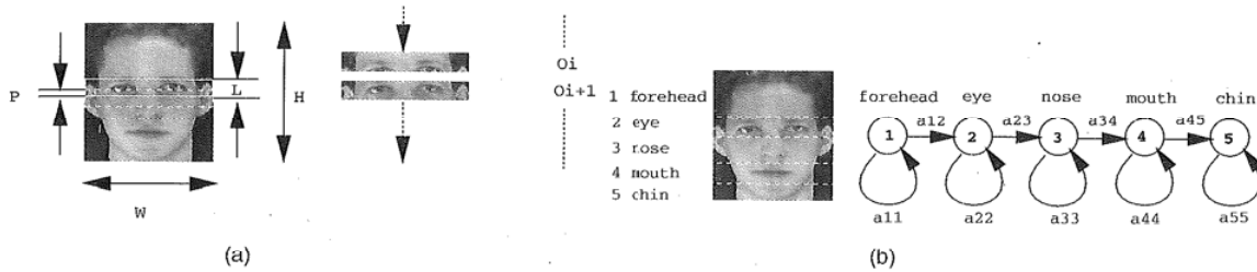
Fig. 11. Hidden Markov model for face localization. (a) Observation vectors: To train an HMM, each face sample is converted to a sequence of observation vectors. Observation vectors are constructed from a window of W \times L pixels. By scanning the window vertically with P pixels of overlap, an observation sequence is constructed. (b) Hidden states: When an HMM with five states is trained with sequences of observation vectors, the boundaries between states are shown in (b) [136].
