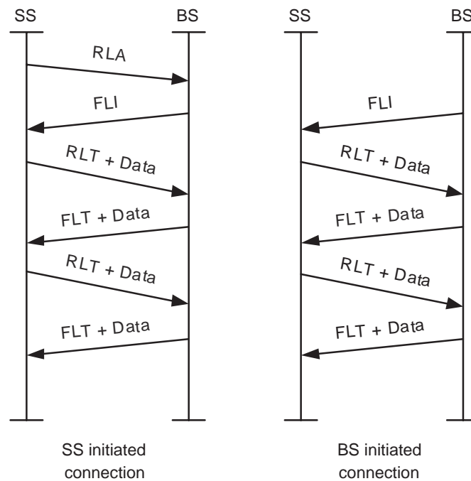
Figure 229—PHY control signal sequence diagrams
