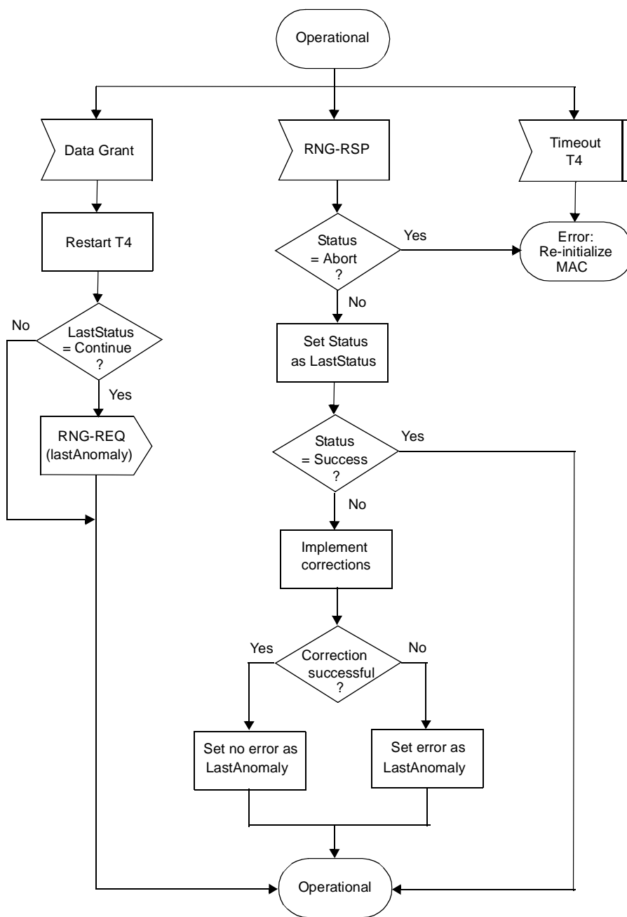
Figure 84—Periodic Ranging—SS
