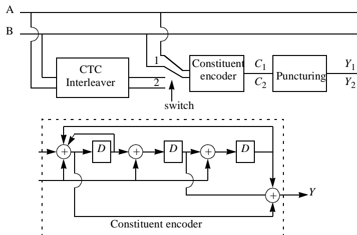
Figure 169—CTC encoder
