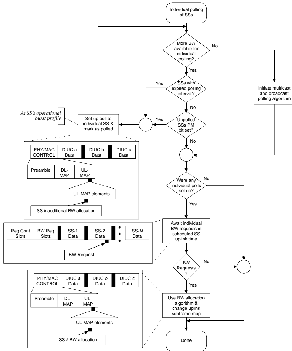
Figure 38—Unicast polling
