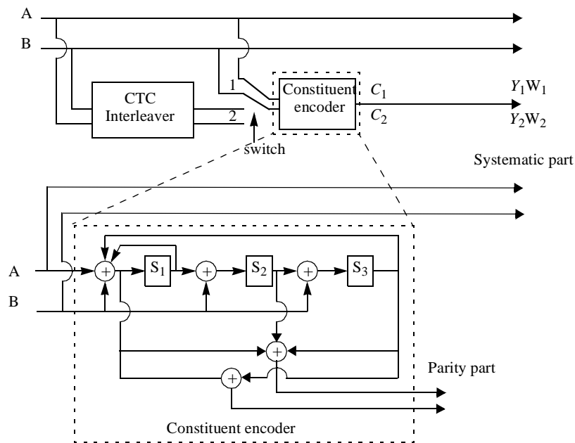
Figure 257—CTC encoder
