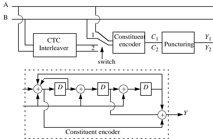
Figure 169—CTC encoder
