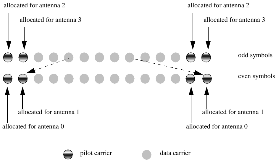
Figure 251—Cluster structure
