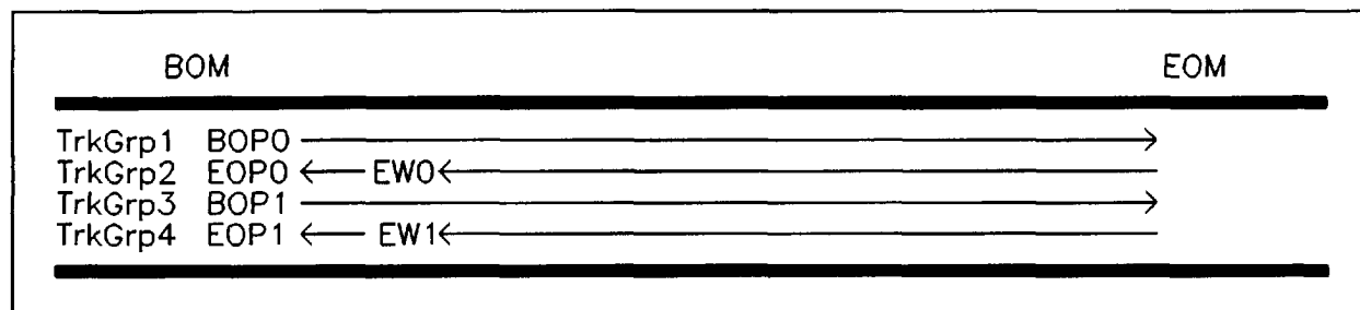
Figure 25 - Partitioning example - one partition per two track groups
