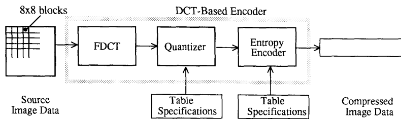
Figure 1. DCT-Based Encoder Processing Steps
