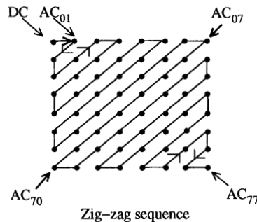
Figure 3. Preparation of Quantized Coefficients for Entropy Coding
