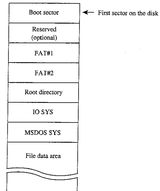
Figure 2-4 Boot-disk configuration
