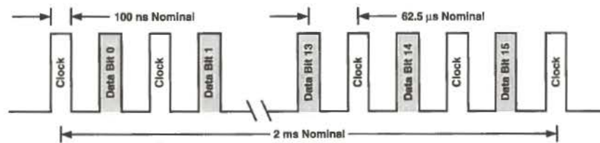
Figure 8-3 Auto-Negotiation signaling.
