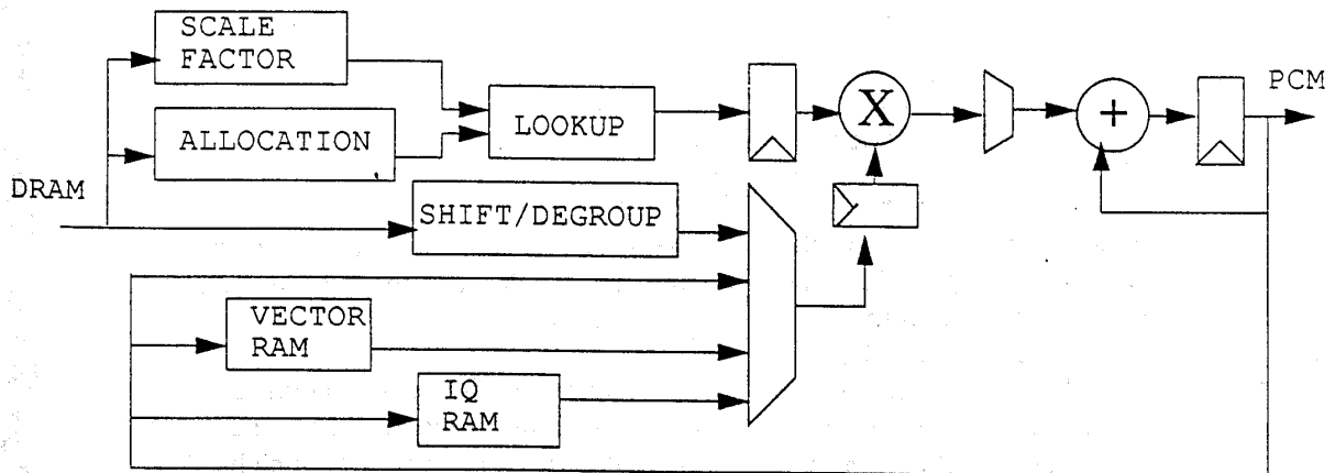
Figure 3. Decoder Architecture
