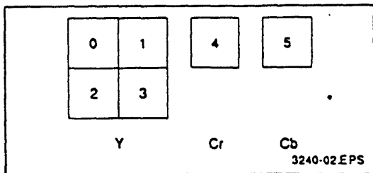
Figure 2 : Macroblock Structure
