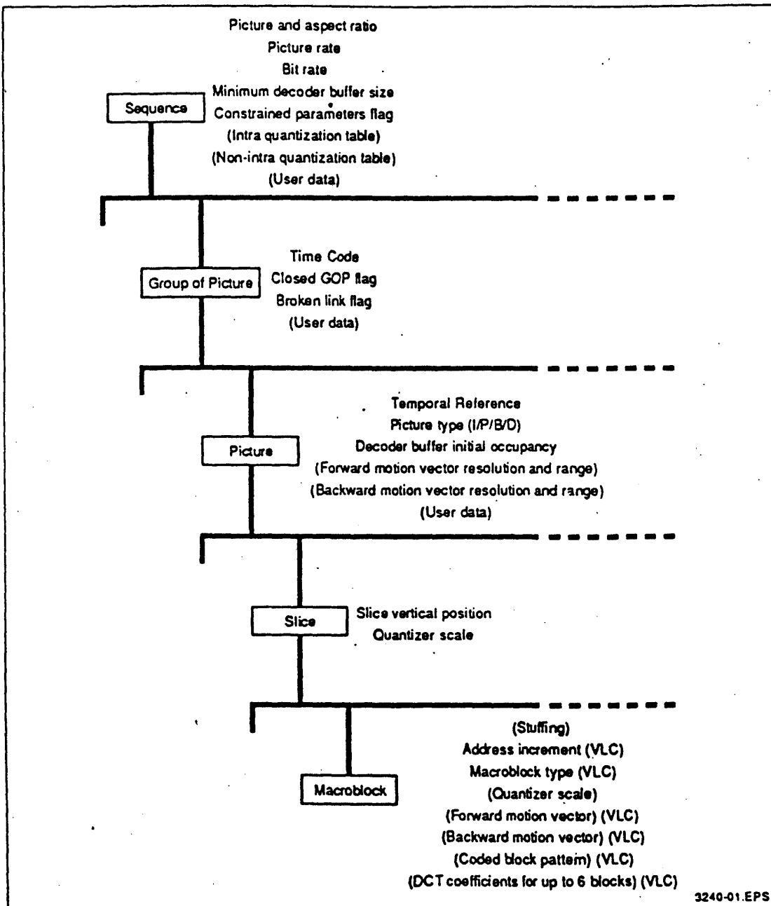
Figure 1 : MPEG Bistream.Hierarchy
