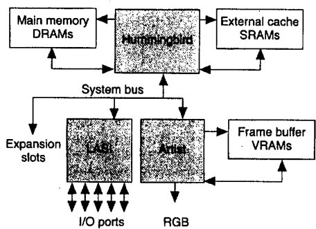
Figure 1. Model 712/60 block diagram.
