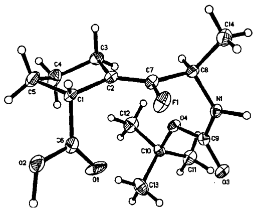
Fig. 1. ORTEP drawing of the x-ray structure of (Z) - l -Boc-Ala- \beta [CF=C]-Pro ( l -3).
