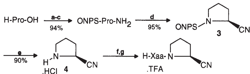
Scheme I. Preparation of dipeptide nitriles.
