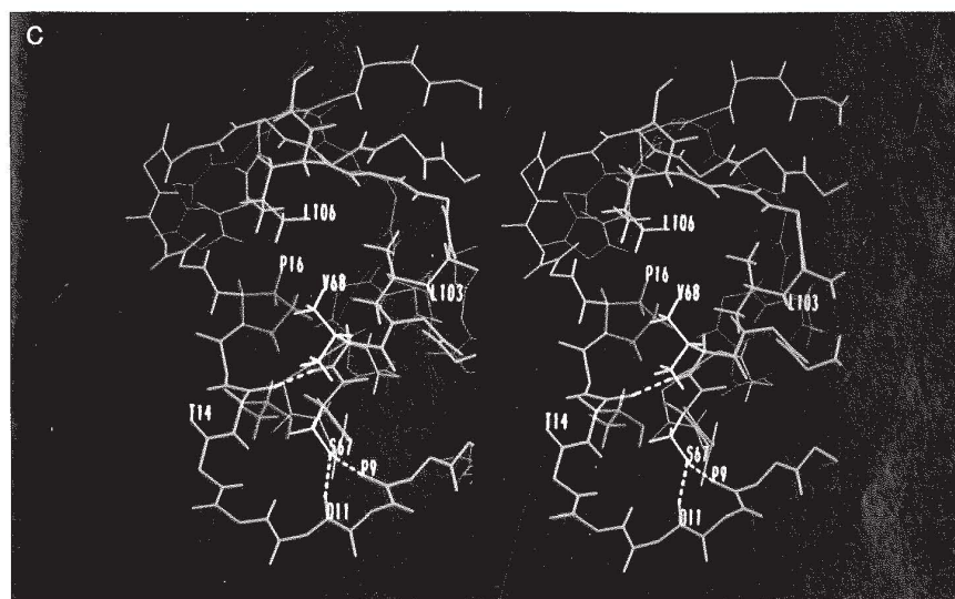
Fig. 2. (A) The \alpha -carbon traces of 13 structures generated by restrained molecular dynamics are shown in blue. \langle SA \rangle_{ref} , which includes side chains of aromatic residues in the drug-binding pocket, is shown as the heavy line. Aromatic side chains are color-coded: Trp, yellow; Phe, orange; and Tyr, green. The NH_2 - and COOH -termini are indicated with green and red dot surfaces, respectively. (B) \langle SA \rangle_{ref} , showing location of the ligand binding site formed by the \beta sheet and the \alpha helix; certain residues are numbered. (C) Expanded view of \langle SA \rangle_{ref} , showing crossing of the loops connecting the first and fourth (relevant residues in orange) and the fifth and second (relevant residues in yellow) strands of the \beta sheet; known interstrand hydrogen bonds are indicated. Relevant residues in the third strand are shown in green. (D) Hydrophobic residues in the drug-binding pocket of \langle SA \rangle_{ref} . Side chains are color-coded as in (A), with additional aliphatic residues in purple.
