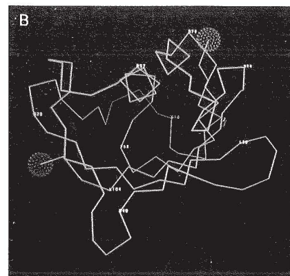
Fig. 2. (A) The \alpha -carbon traces of 13 structures generated by restrained molecular dynamics are shown in blue. \langle SA \rangle_{ref} , which includes side chains of aromatic residues in the drug-binding pocket, is shown as the heavy line. Aromatic side chains are color-coded: Trp, yellow; Phe, orange; and Tyr, green. The NH_2 - and COOH -termini are indicated with green and red dot surfaces, respectively. (B) \langle SA \rangle_{ref} , showing location of the ligand binding site formed by the \beta sheet and the \alpha helix; certain residues are numbered. (C) Expanded view of \langle SA \rangle_{ref} , showing crossing of the loops connecting the first and fourth (relevant residues in orange) and the fifth and second (relevant residues in yellow) strands of the \beta sheet; known interstrand hydrogen bonds are indicated. Relevant residues in the third strand are shown in green. (D) Hydrophobic residues in the drug-binding pocket of \langle SA \rangle_{ref} . Side chains are color-coded as in (A), with additional aliphatic residues in purple.
