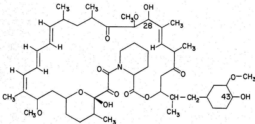
Rapamycin
