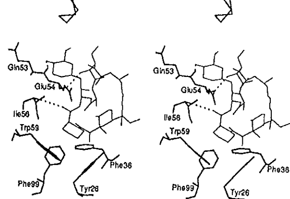
Figure 1. (a, top) A stereoview of the \alpha -carbon tracing of FKBP-12 and rapamycin. The N- and C-terminal \alpha -carbons are labeled. (b, bottom) A stereodrawing of the binding pocket showing all of the bound rapamycin molecule and selected FKBP-12 residues.
