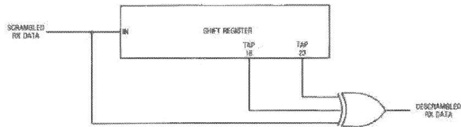
Fig 11-12 Descrambler
