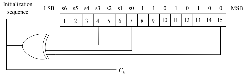
Figure 243—PRBS generator for ranging code generation
