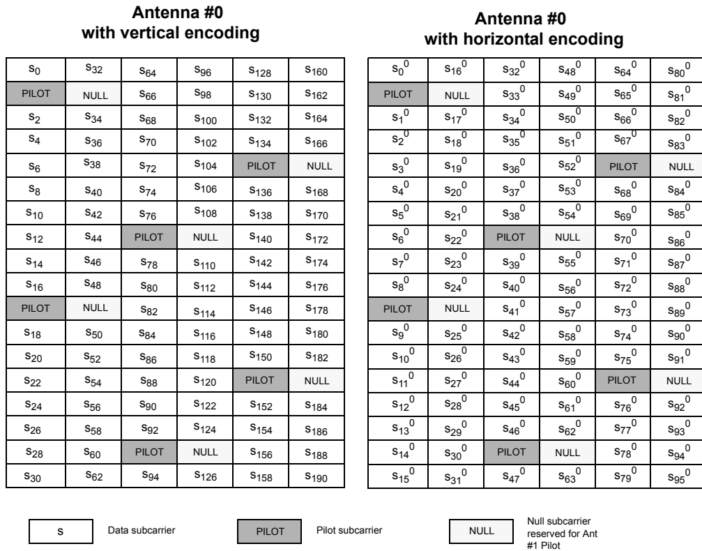
Figure 251j—Data mapping in the optional AMC zone with 2 Tx antenna and matrix B
