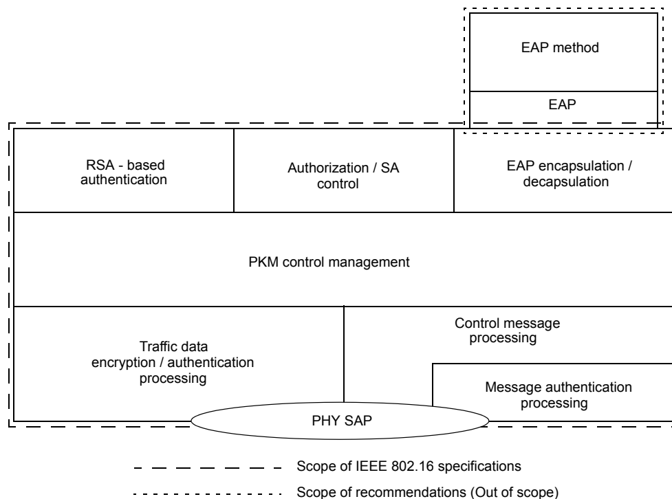
Figure 130j—Security sublayer
