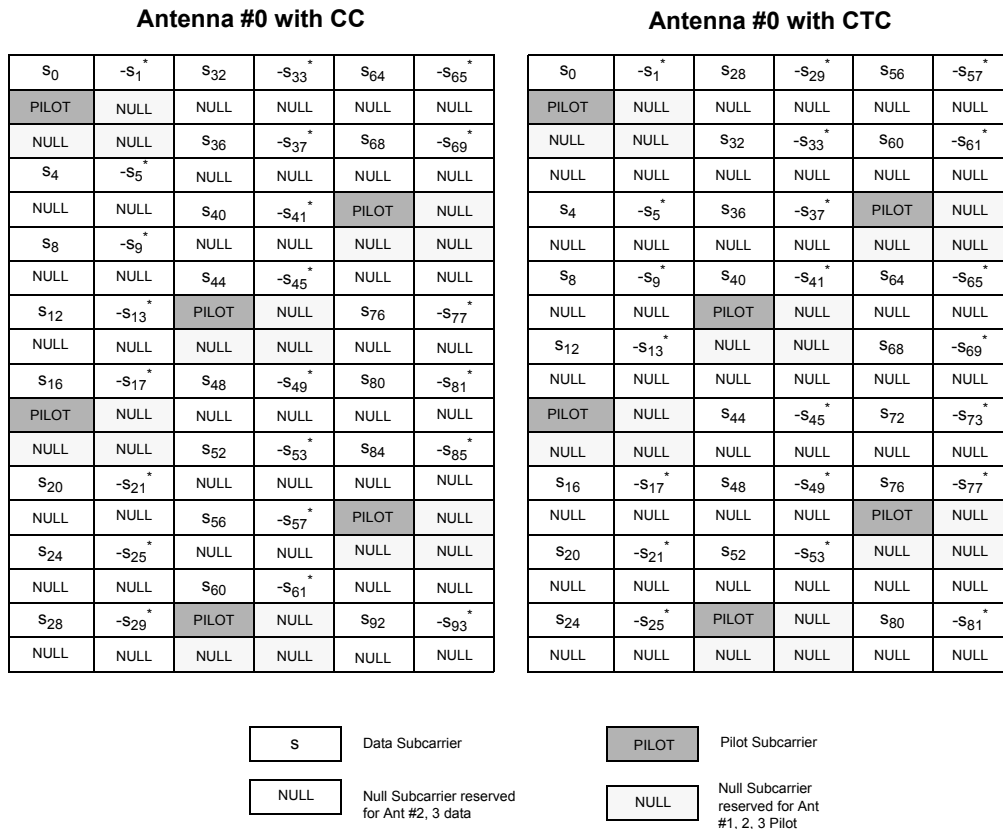
Figure 251k—Data mapping with CC in the optional AMC Zone with 4 Tx antenna and Matrix A
