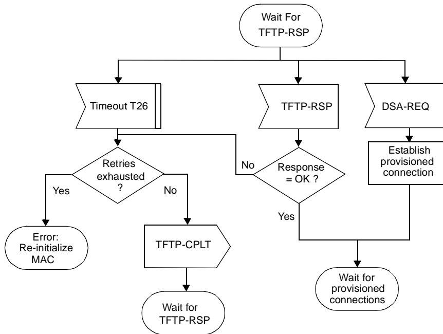
Figure 72—Wait for TFTP-RSP—SS
