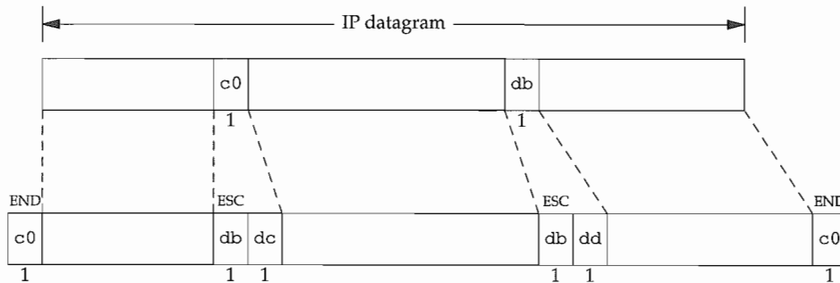
Figure 2.2 SLIP encapsulation.
