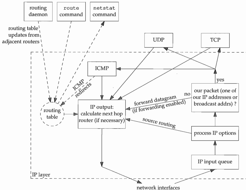
Figure 9.1 Processing done at the IP layer.
