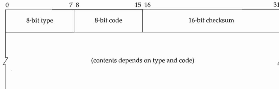
Figure 6.2 ICMP message.
