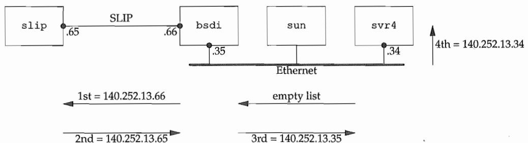
Figure 7.4 ping with record route option.
