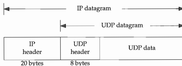
Figure 11.1 UDP encapsulation.
