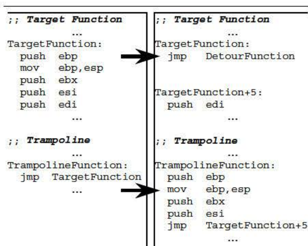
Figure 2. Trampoline and target functions, before and after insertion of the detour (left and right).
