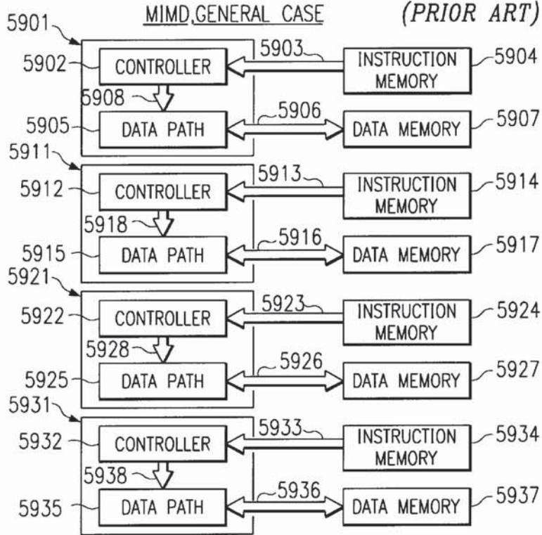
FIG. 60 (PRIOR ART)
