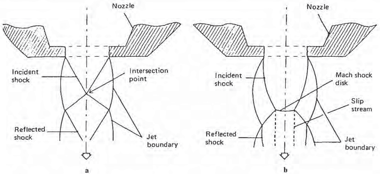
Figure D1.2.6. Shock structures in a supersonic jet: (a) regular intersection; (b) at higher pressures the formation of a Mach shock disc [10, 11].
