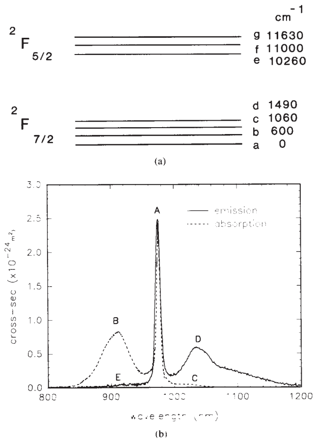
Fig. 1. (a) The Yb 3+ energy level structure, consisting of two manifolds, the ground manifold 2 F 7/2 (with four Stark levels, labeled (a)–(d)), and a well separated excited manifold 2 F 5/2 (with three Stark levels labeled (e)–(g)). Approximate energies in wavenumbers above ground energy are indicated. (b) Absorption and emission cross sections for a germanosilicate host. The principal features of the spectra have been labeled A–E, and are discussed in the text.
