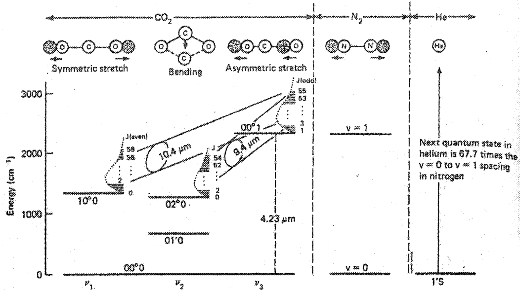
Figure 12.3 Laser states of the carbon dioxide molecule. (From LASER ELECTRONICS 2E, by VERDEYEN, J.T. ©1989, Figure 10.14, p. 336. Adapted by permission of Prentice-Hall, Inc., Upper Saddle River, NJ.)
