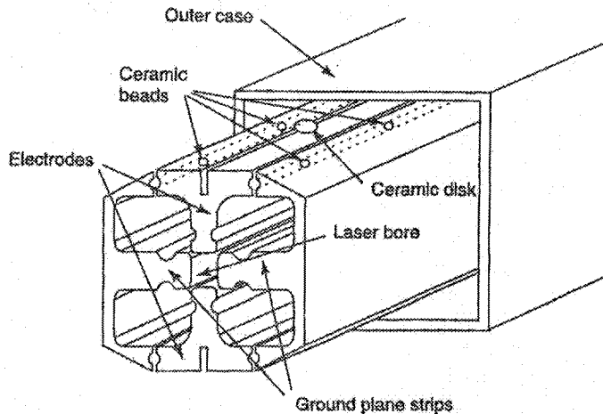
Figure 12.13 The Synrad series 48 cross-section.
