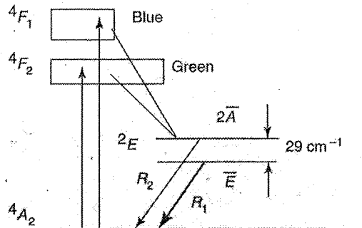
Figure 11.2 The energy band diagram for ruby.
