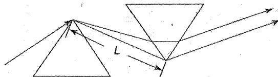
Figure 11.26 Prisms are the most common way of introducing GVD compensation. A prism geometry can be arranged so that the blue components transverse the prism path in a shorter length of time than the red components.
