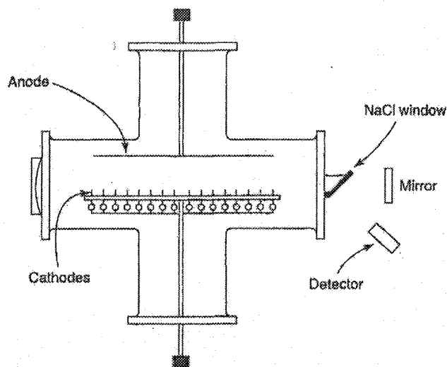
Figure 12.6 A schematic of an early Transverse Excited Atmospheric (TEA) laser. (Reprinted with permission from A. J. Besulieu, Appl. Phys. Lett. 16:504 (1970). ©1970 American Institute of Physics.)
