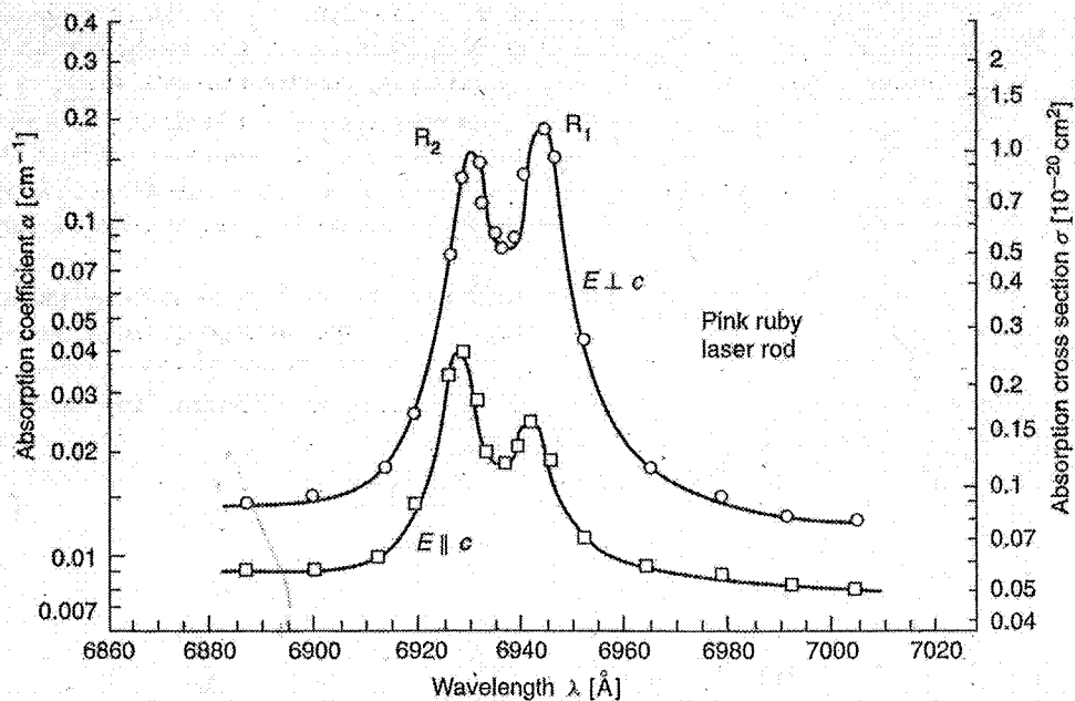
Figure 11.3 Since ruby is uniaxial, its absorption coefficient is a very strong function of the polarization direction of the light. (From D. C. Cronmeyer, J. Opt. Soc. Am. 56:1703 (1966). Reprinted with the permission of the Optical Society of America.)
