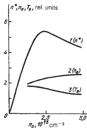
FIG. 1. Dependence of the parameters of a cesium plasma on the density of Cs vapor at fixed intensity of resonance irradiation. 18 1—density n^* of excited atoms ( \text{Cs}, 8^2P ); 2—density n_e of electrons; 3—temperature T_e of electrons.
