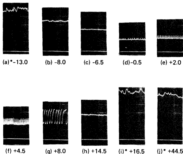
FIG. 5. Time variation of the transmitted laser beam (of power fixed at 170 mW) through the Cs vapor at 380 °C. The numbers indicated in (a) to (j) are detuning of the laser (in GHz) from the center of the absorption line. No plasma is formed in (a), (i), and (j) (denoted by asterisk). On the low-frequency wing [i.e., (b) and (c)] QRLPP is formed and noise reduction is observed in the transmitted beam. Near line center and on the high-frequency wing, (d)–(g), self-oscillation of the QRLPP occurs. For large positive detuning (h), no self-oscillation in the QRLPP is observed, but the plasma is “metastable”, i.e., it is destroyed when the cw laser is momentarily interrupted. The horizontal time scale is 10 msec/cm, and the vertical scale (proportional to laser intensity) is constant in each scope picture, with the zero line given near the bottom.
