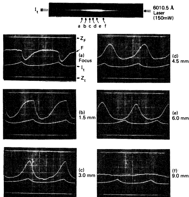
FIG. 7. Transmitted laser intensity ( I_t ) and fluorescence intensity ( F ) at various positions in the QRLPP. (a) gives F at the laser focus, while (b)–(f) give F at increasing distance upstream from the laser focus (the distance is indicated). The Cs density is fixed at 1.8 \times 10^{17} \text{ cm}^{-3} .
