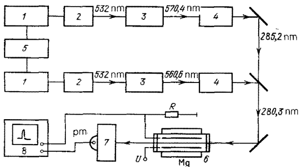
FIG. 7. Diagram of an experimental arrangement to form a quiresonance laser plasma in Mg vapor. 36 1—neodymium garnet laser; 2, 4—frequency doublers based on KDP; 3—dye laser; 5—delay circuit; 6—cell with Mg vapor; 7—monochromator with photomultiplier (PM); 8—oscillograph.
