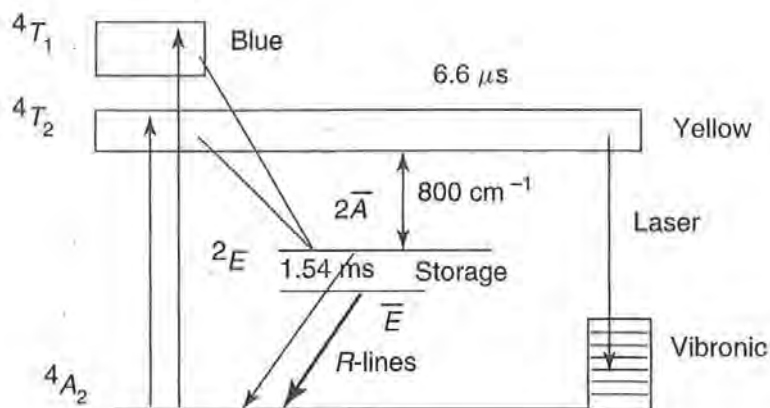
Figure 11.4 The energy band diagram for alexandrite.
