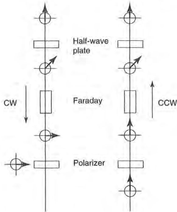
Figure 11.17 The contrasting properties of Faraday rotators and half-wave plates allow the creation of an optical diode. This system passes CCW light unchanged, but attenuates CW light.
