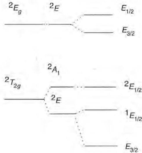
Figure 11.6 The energy band diagram for Ti:sapphire.
