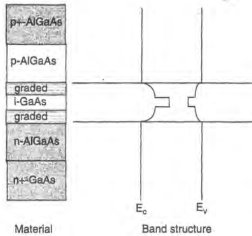
Figure 12.39 A GRINSCH laser is basically a DH laser, but one where the higher bandgap layer has been graded to meet the lower bandgap layer. This provides both electron confinement (from the energetic well created by the graded bandgap) and optical confinement (from the index of refraction bump between the high and low index materials).
