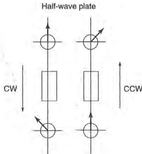
Figure 11.14 Vertically polarized light passing through a half-wave plate in clockwise (CW) and counter-clockwise (CCW) directions.
