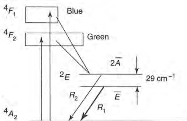
Figure 11.2 The energy band diagram for ruby.
