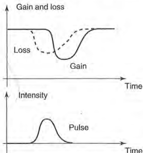
Figure 11.27 In lasers where the upper state lifetime is short in comparison to the cavity round-trip time, there is a window between the drop in loss due to the dye bleaching and the drop in gain due to dynamic gain saturation. This window favors the more intense pulse.
