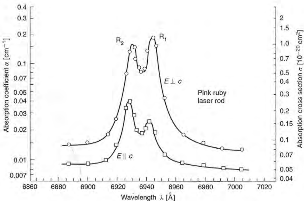
Figure 11.3 Since ruby is uniaxial, its absorption coefficient is a very strong function of the polarization direction of the light. (From D. C. Cronmeyer, J. Opt. Soc. Am. 56:1703 (1966). Reprinted with the permission of the Optical Society of America.)
