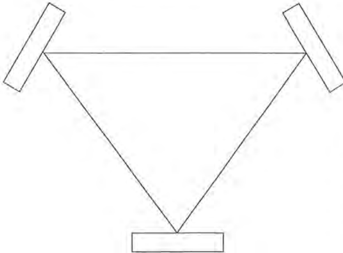
Figure 11.9 A simple ring resonator will have longitudinal modes (the back-and-forth length of a conventional laser is equivalent to the round-trip length of a ring laser) and standing wave patterns (formed by the interaction between the left and right traveling waves in the ring).
