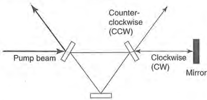
Figure 11.11 One method for generating unidirectional oscillation in a ring laser is to create a small external cavity aligned with one of the propagating directions of the ring laser.
