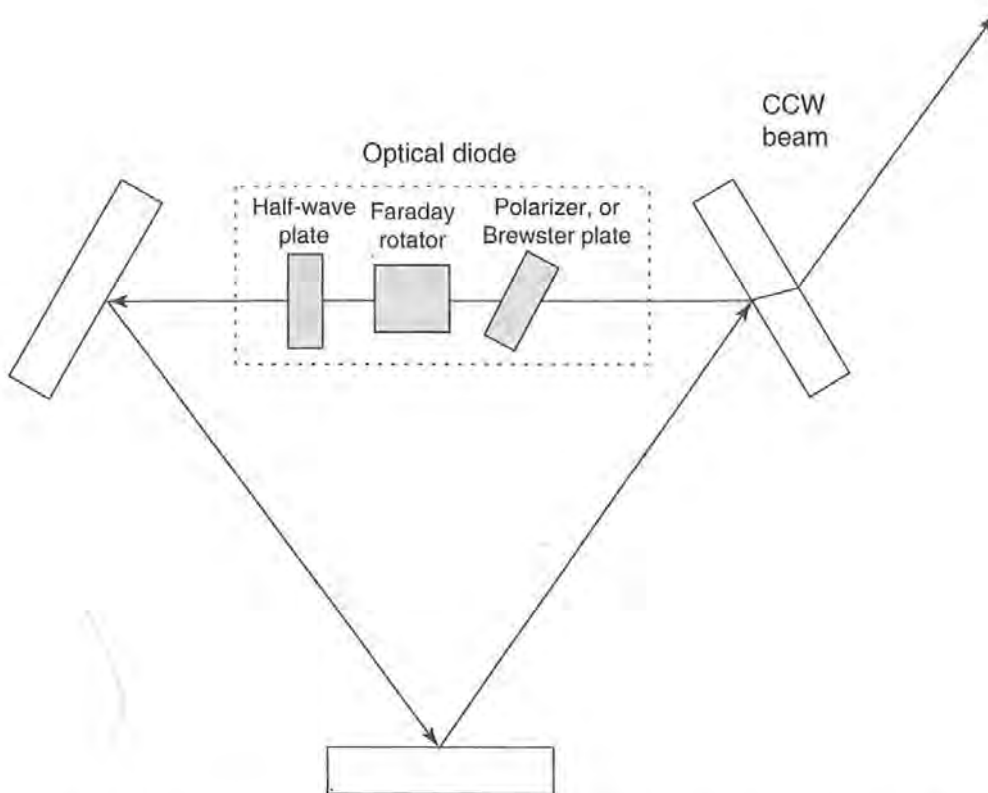
Figure 11.12 Another method for generating unidirectional oscillation in a ring laser is to place an optical diode (constructed from a Faraday rotator, a half-wave plate, and a Brewster plate or polarizer) in the resonator.
