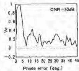
Fig. 5. Phase comparator characteristic.
