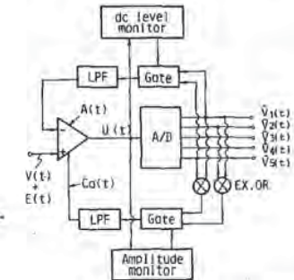
Fig. 7. Feedback circuit configuration.
