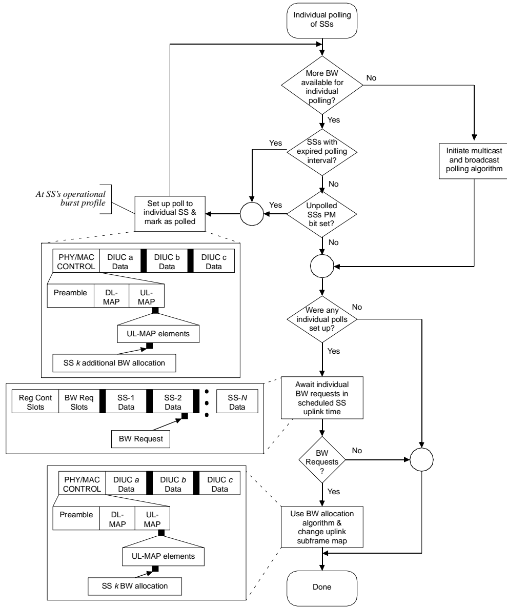
Figure 38—Unicast polling
