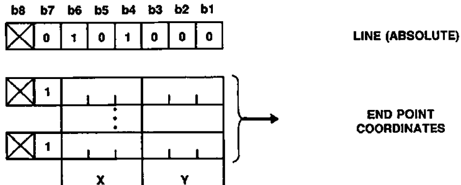
Figure 36 LINE (Absolute)
