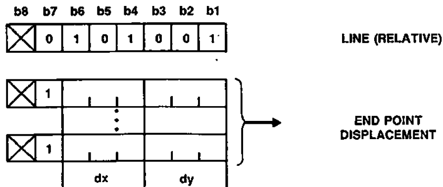
Figure 37 LINE (Relative)
