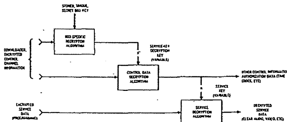
Figure 4. Multilevel Key Distribution (Decoder End)
