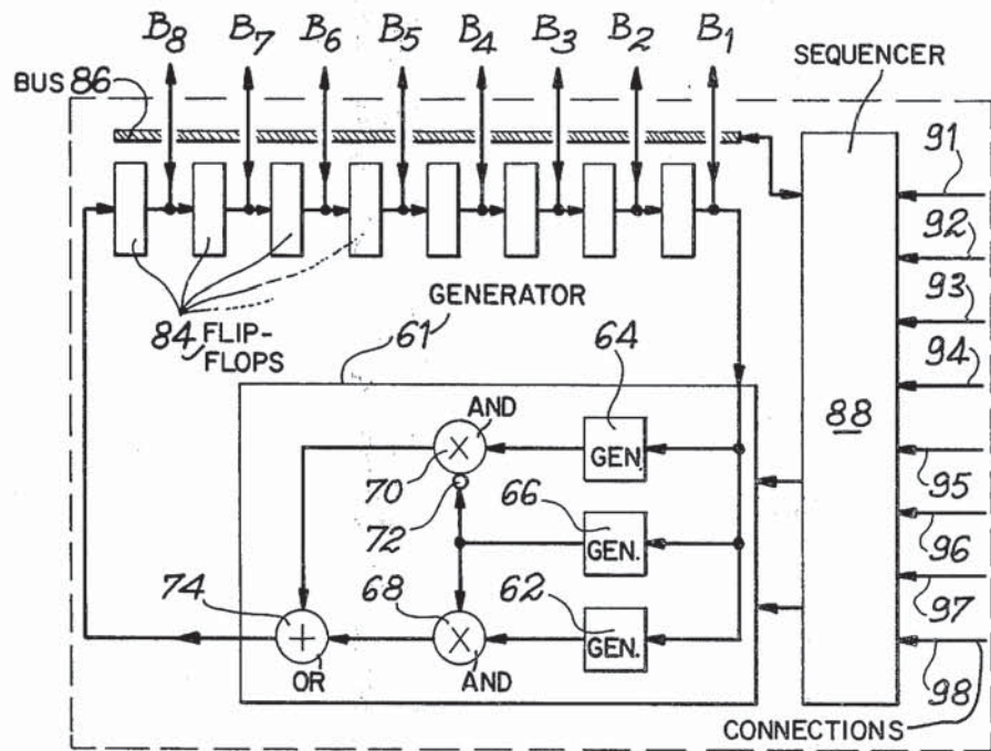
FIG. 5 GENERATOR 26 (26')
