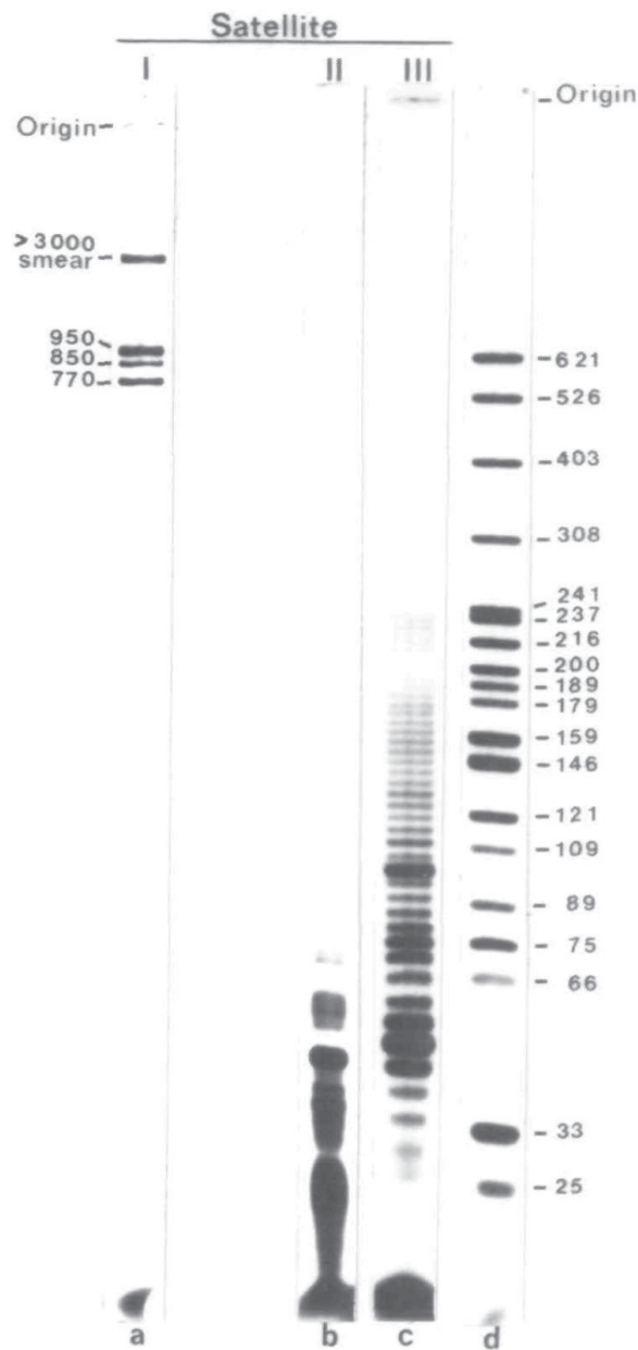
Figure 1. 4% polyacrylamide gels of [\alpha\text{-}^{32}\text{P}]\text{ATP} -labelled fragments produced by digestion of satellites I, II and III with HinfI.
