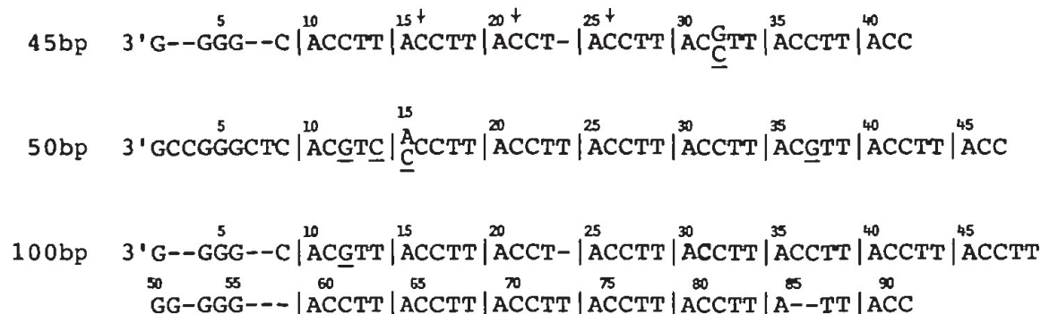
Figure 7. Base sequences of the 45bp, 50bp and 100bp HinfI fragments of satellite III. The 5bp monomers, 5' TTCCA, are marked and positions where the consensus sequence has clearly diverged from the monomer sequence are underlined. Positions where the consensus sequence could not be easily read are left blank. Positions in the 45bp sequence where a single base change would generate a HinfI and TaqI site are marked with arrows. The 100bp fragment is presented as two tandem repeats of 49bp each.
