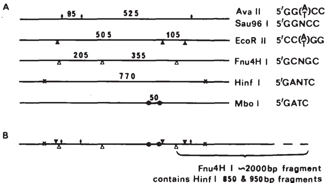
Figure 6. Restriction site map of satellite I.
