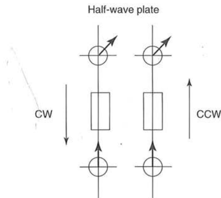
Figure 11.16 Vertically polarized light passing through a half-wave plate in the CCW direction, being back-reflected, and passing back through the half-wave plate in the CW direction.
