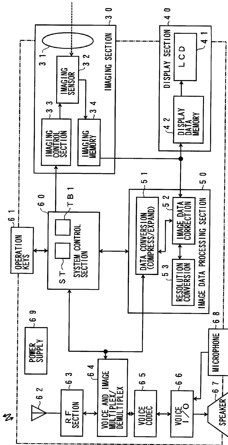
FIG. 2 1.2 PORTABLE TERMINAL
