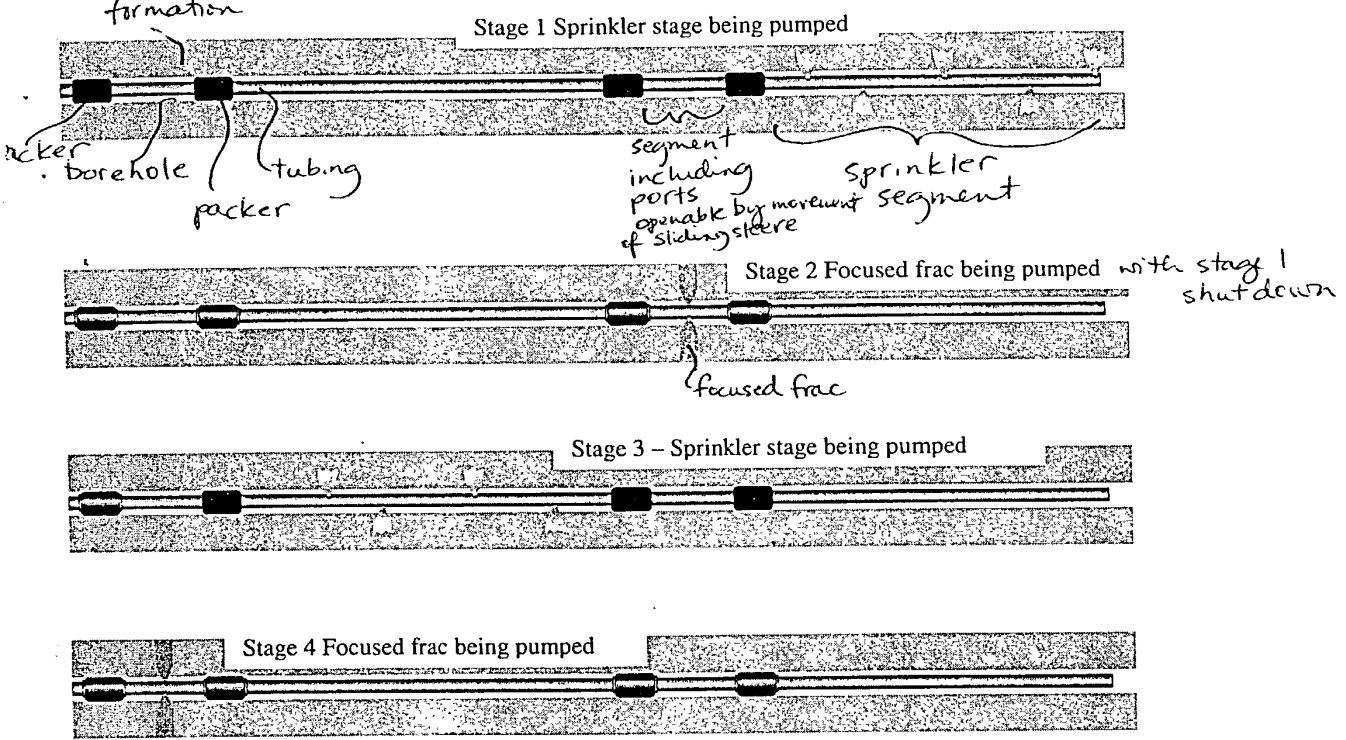
Figure 3 Multi-stage Frac and Sprinkler System
