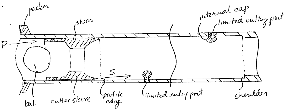
stage 2 tubing in cross section
