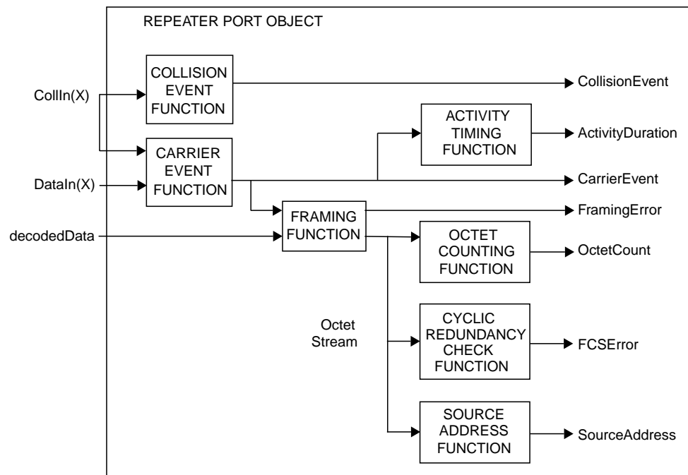
Figure 30-2—Functions relationship
