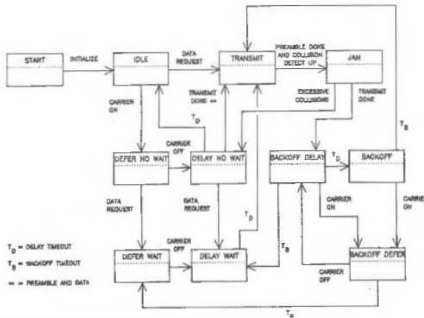
Fig B1 Transmit Component State Diagram
