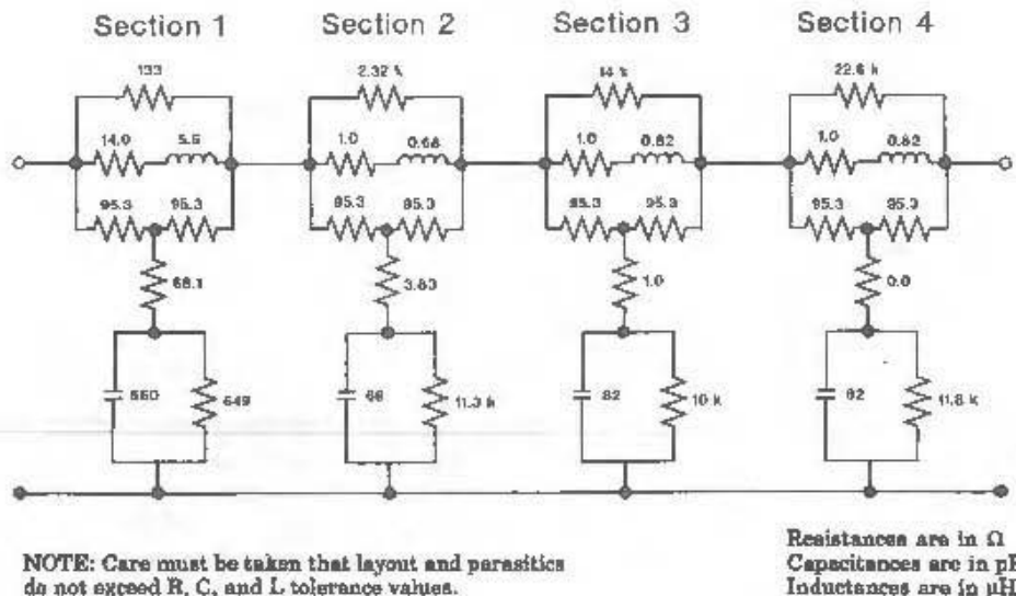
Fig 14-7 Twisted-Pair Model
