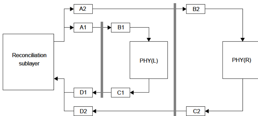
Figure 22A-3—Combined model
