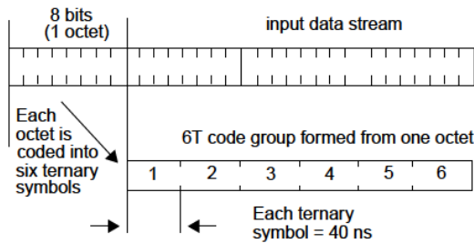
Figure 23-4—8B6T coding
