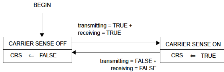
Figure 24-12—Carrier Sense state diagram
