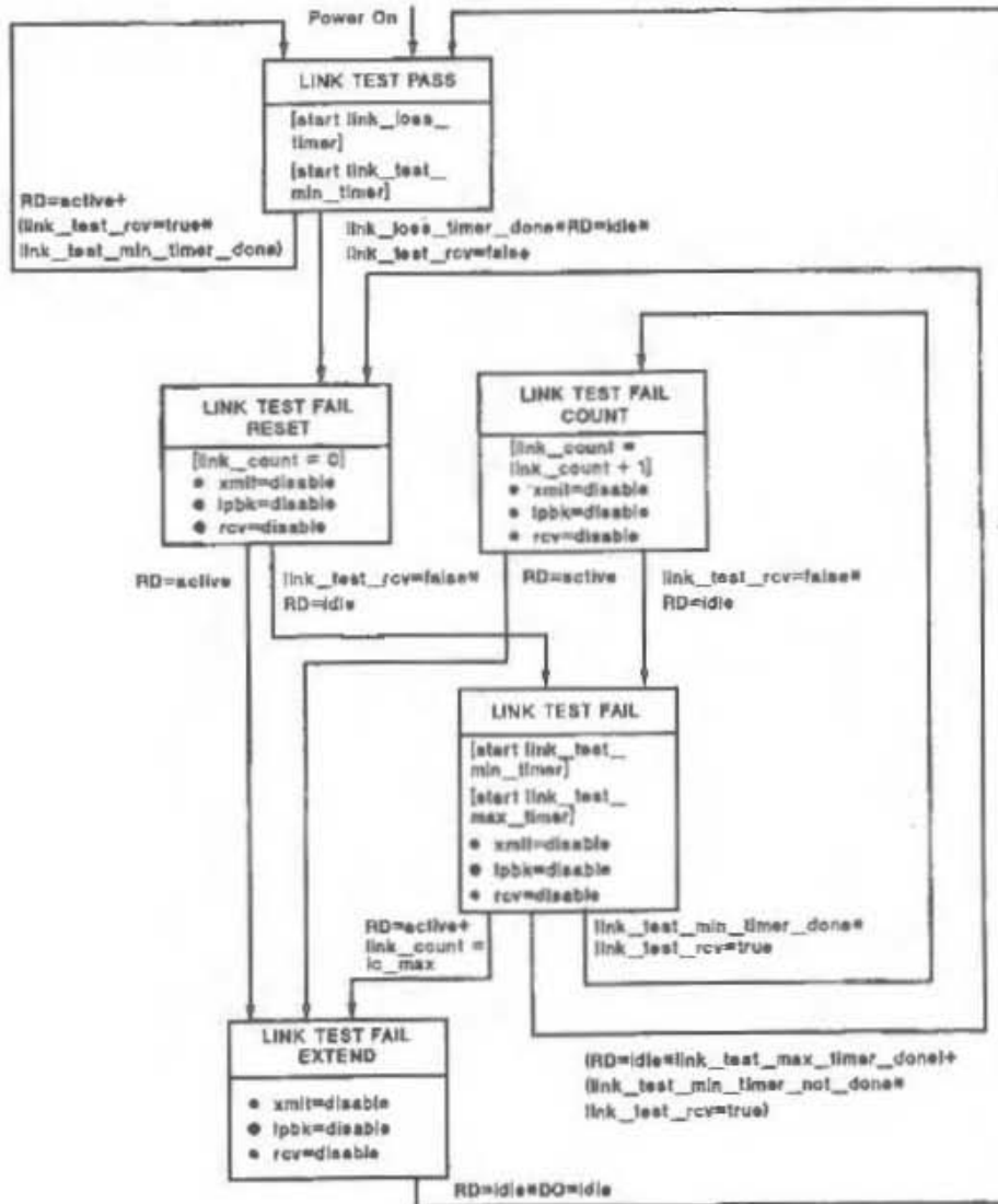
Fig 14-6 Link Integrity Test Function State Diagram
