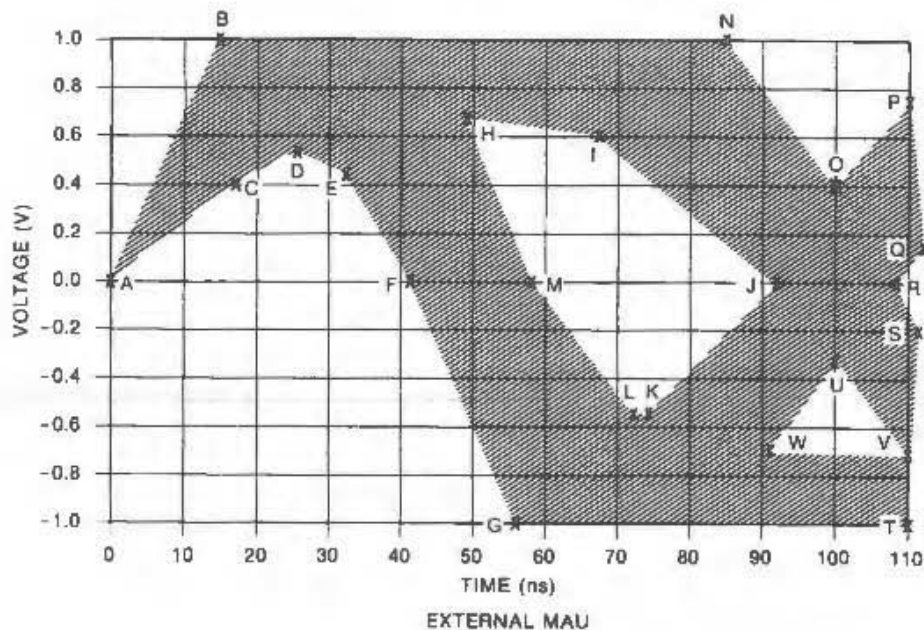
Fig 14-9 Voltage Template
