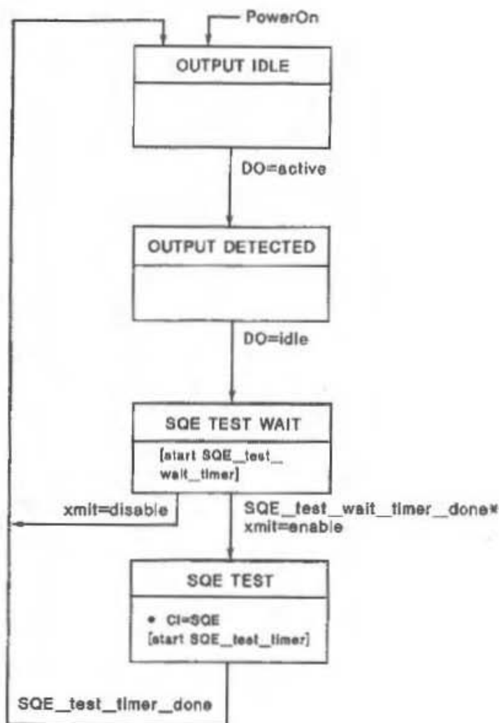
Fig 14-4 signal_quality_error Message Test Function State Diagram
