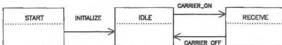
Fig B2 Receive Component State Diagram
