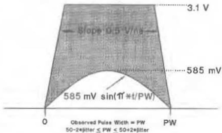
Fig 14-16 Receive Differential Input Voltage—Narrow Pulse
