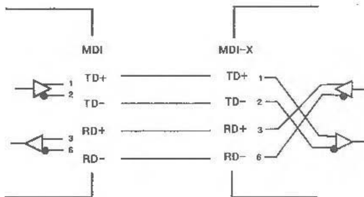
(b) MAU-Embedded Crossover Function
