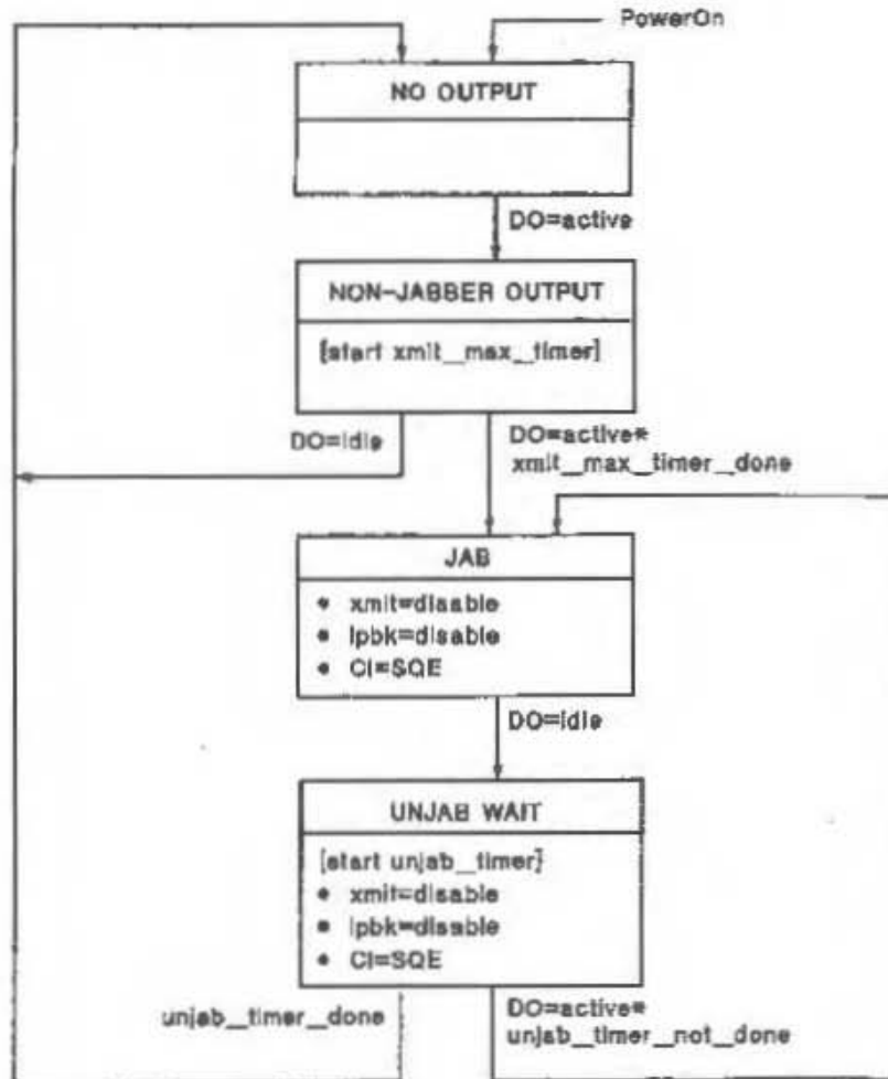
Fig 14-5 Jabber Function State Diagram
