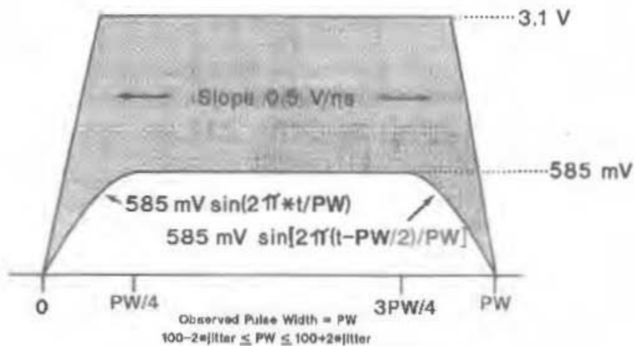
Fig 14-17 Receiver Differential Input Voltage—Wide Pulse
