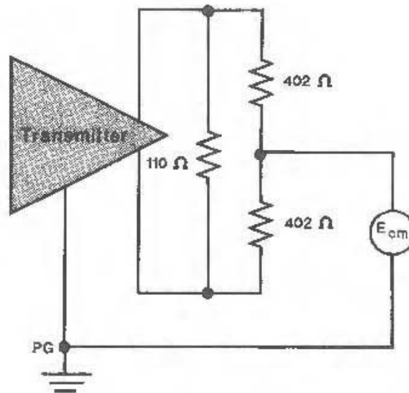
Fig 14-15 Transmitter Fault Tolerance Test Circuit
