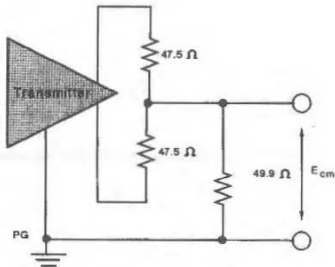
Fig 14-14 Common-Mode Output Voltage Test Circuit
