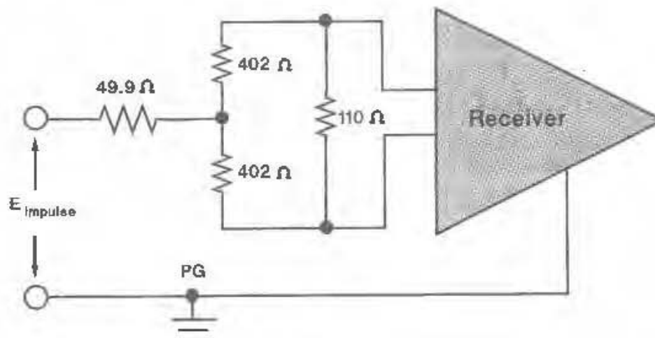
Fig 14-19 Common-Mode Impulse Test Circuit
