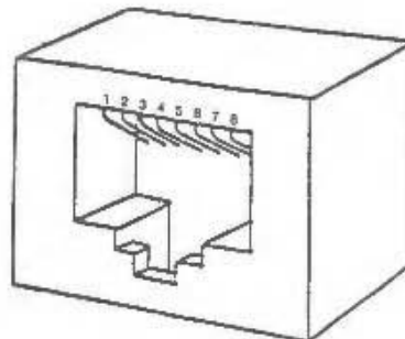
Fig 14-20 MAU MDI Connect
