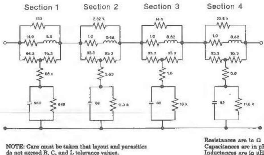
Fig 14-7 Twisted-Pair Model
