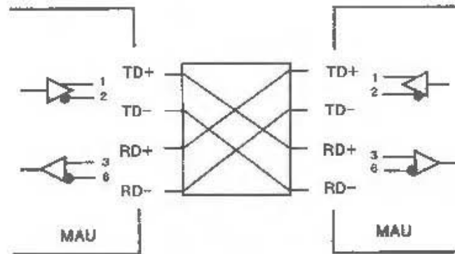
(a) External Crossover Function
