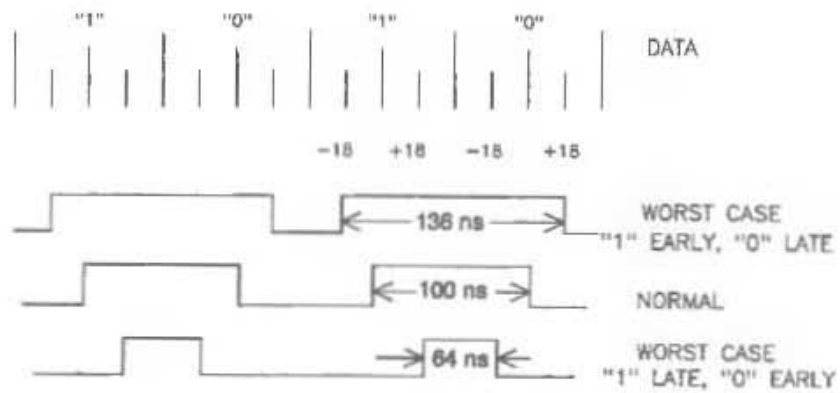
Fig A3 Worst-Case Signal Waveform Variations
