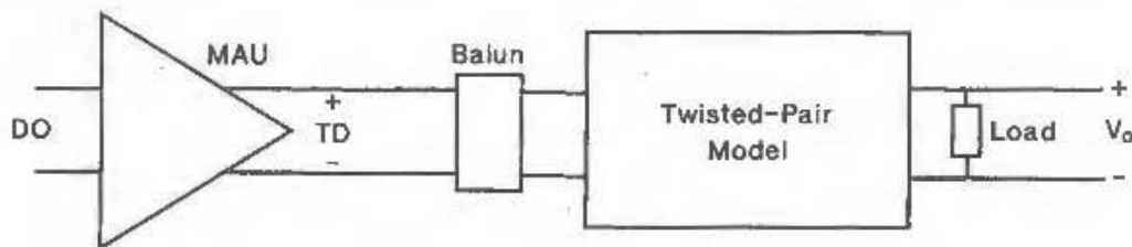
Fig 14-8 Differential Output Voltage Test
