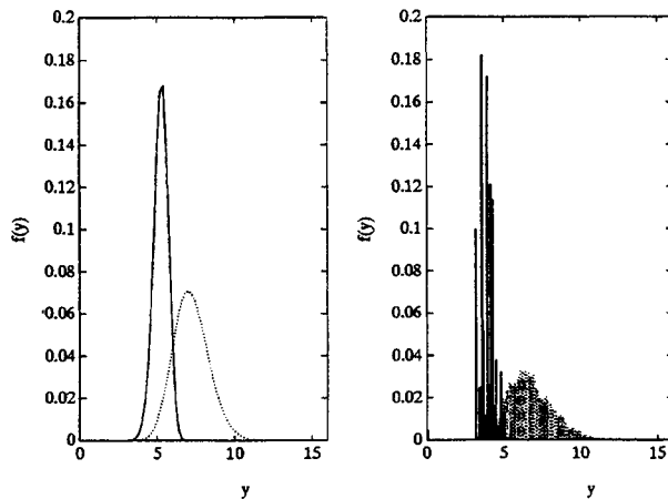
Figure 3: Density functions f_{P_x}(y) (dotted) and f_{min}(y) (solid) for \sigma^2 = 0.09 , N = 80 , and L_w = 20 (left graph) and corresponding histograms of \bar{P}_x(i) (dotted) and P_n(i) (solid) for car noise signals (right graph)
