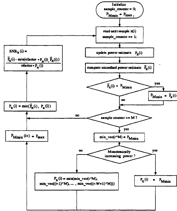
Figure 2: Flowchart of the SNR estimation algorithm
