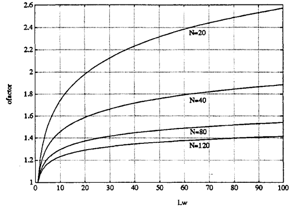
Figure 4: Overestimation factor ofactor versus N and L_w
