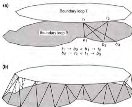
Fig. 20.4 An example of two planar, parallel isoline loops connected to form a triangulated solid: (a) the shortest span method of surface triangulation; (b) surface triangulation of two boundary layers.
