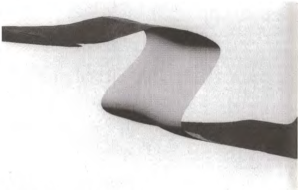
Fig. 20.6 A view of the two original limbs of the fold structure now connected by the overfold.
